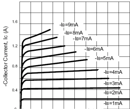
Static Characteristics
