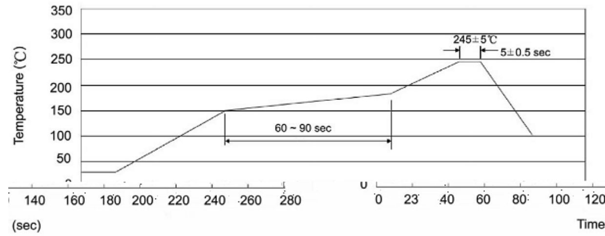
( ) / Temperature Profile for Dip Soldering(Pb-Free)
